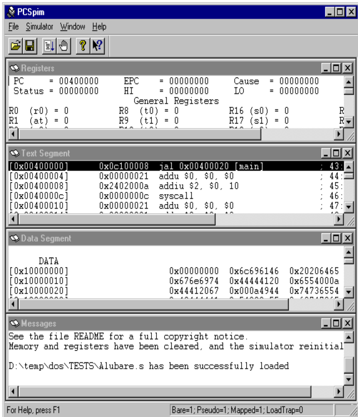
Figure A.1. PCSpim's window interface
